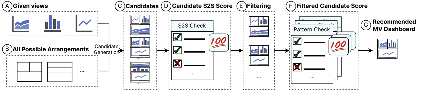
Figure 6. The recommender framework. Given several views and pre-computed possible arrangements, we first generate the candidate dashboards. Then we apply S2S rules to prune unreasonable candidates to improve efficiency. The remaining candidates are further assigned scores and ranked using other rules. Finally, we recommend the candidate with the highest score.
