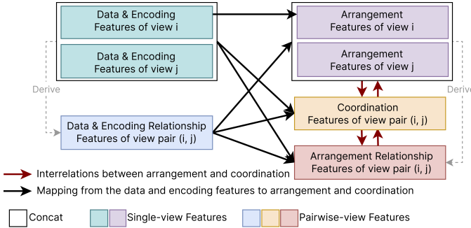
Figure 4. The targeted mappings in our design rule mining. We identified ten mappings in black and red between features in designing dashboards, while the gray dotted lines show the derivation relationship. These black mappings focus on how to utilize data and encoding information of single views for arranging these views in a dashboard and adding coordination among them. The red mappings between arrangement features and coordination features are used to further comprehensively describe the dashboard design.
